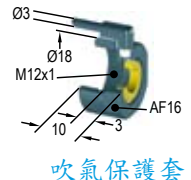
MB12MSC2 (SC75M5-7)
